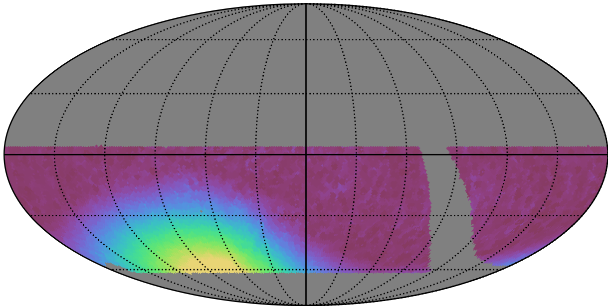
retro_baseline_v2.0_10yrs WFD z band: Min moonDistance
