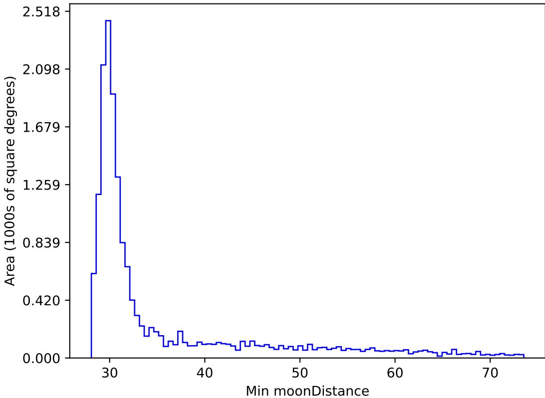
retro_baseline_v2.0_10yrs WFD z band: Min moonDistance
