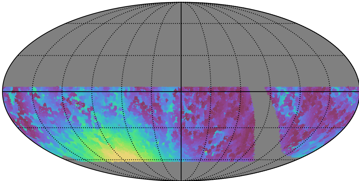
retro_baseline_v2.0_10yrs WFD r band: Min moonDistance
