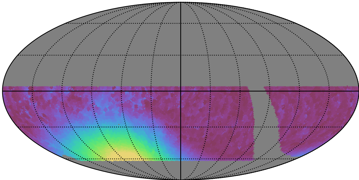
retro_baseline_v2.0_10yrs WFD i band: Min moonDistance
