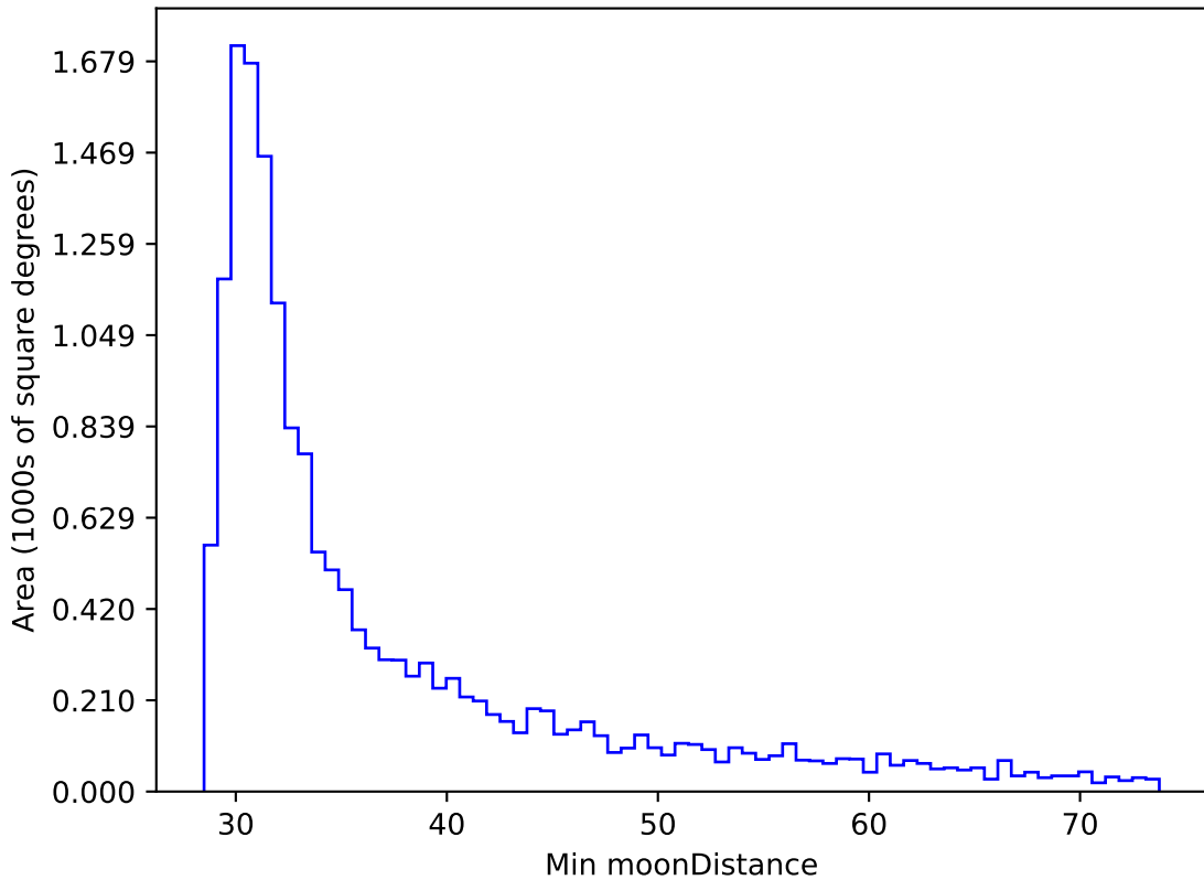
retro_baseline_v2.0_10yrs WFD i band: Min moonDistance
