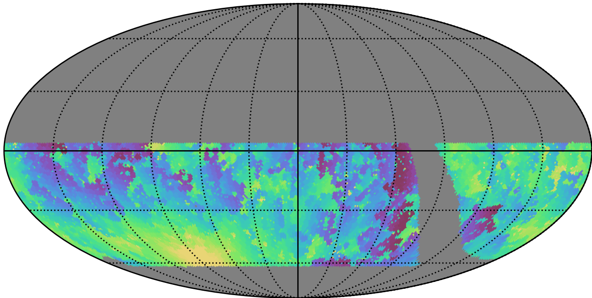
retro_baseline_v2.0_10yrs WFD g band: Min moonDistance
