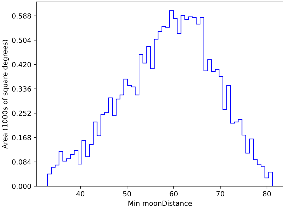
retro_baseline_v2.0_10yrs WFD g band: Min moonDistance
