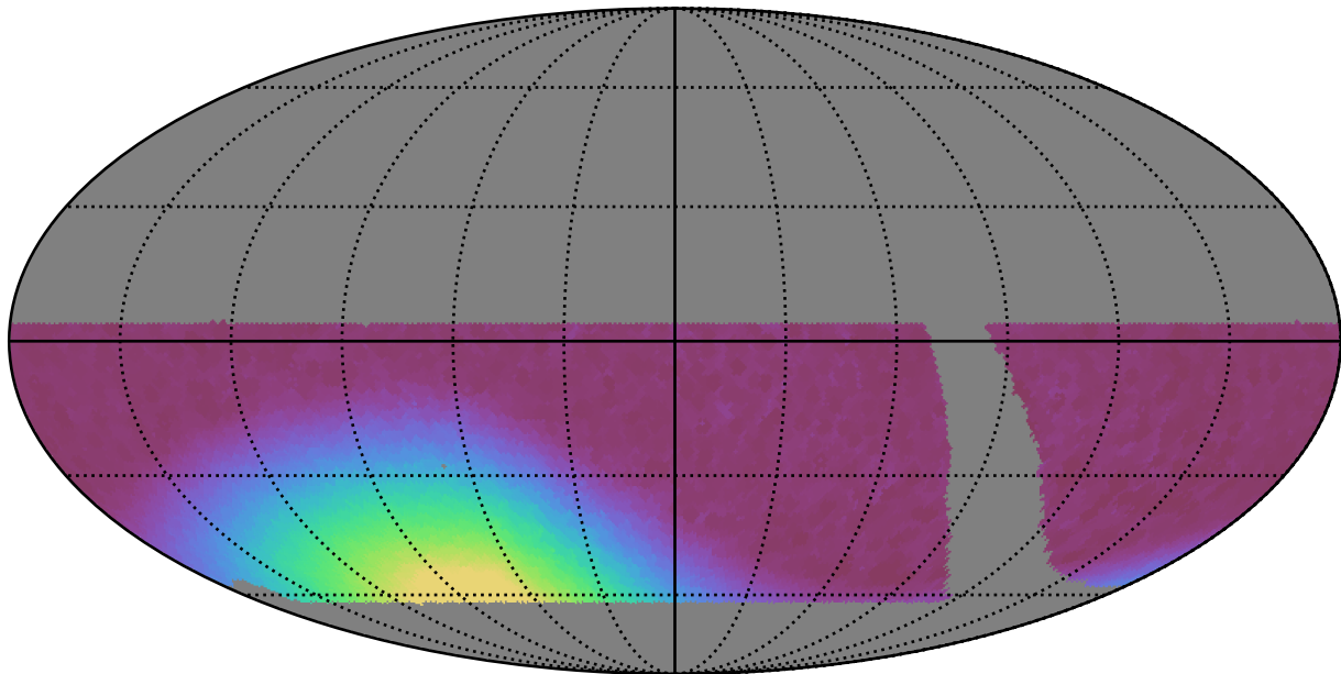
retro_baseline_v2.0_10yrs WFD all bands: Min moonDistance
