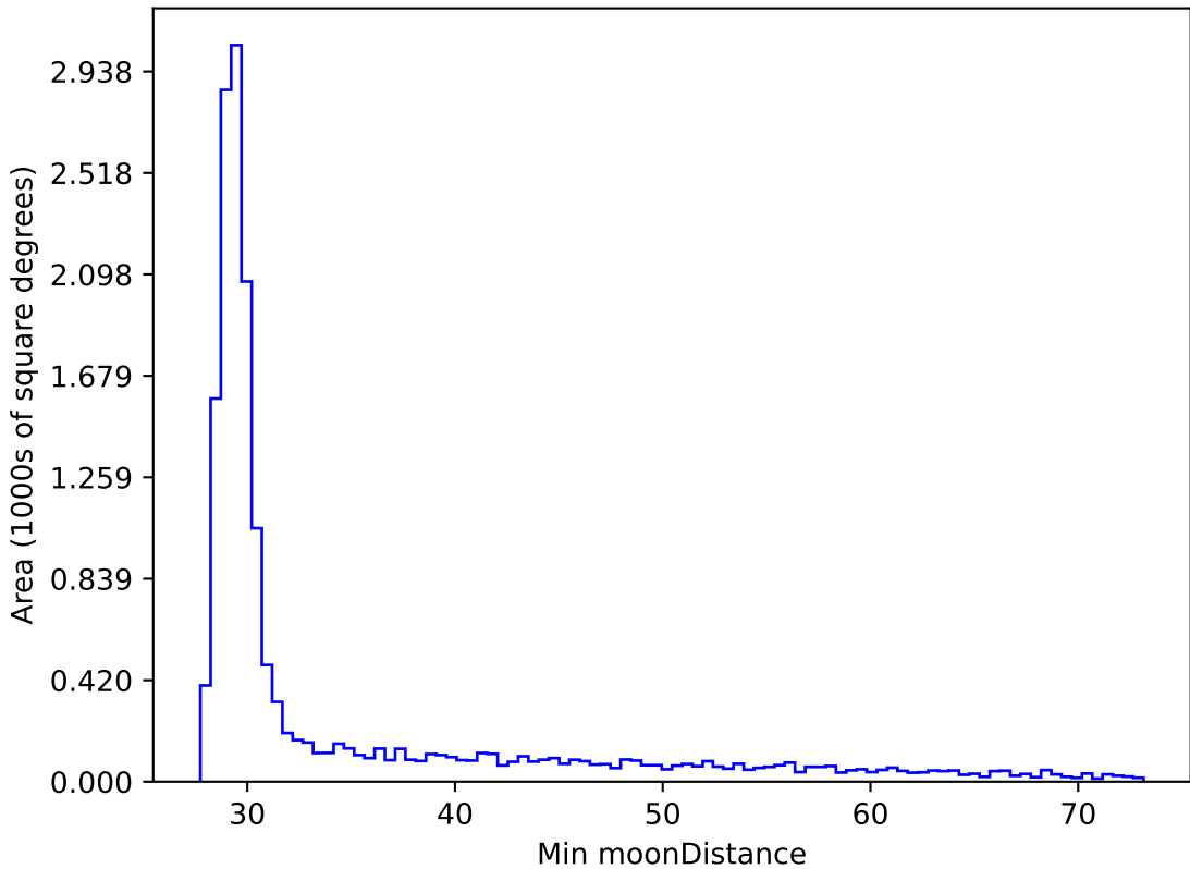
retro_baseline_v2.0_10yrs WFD all bands: Min moonDistance
