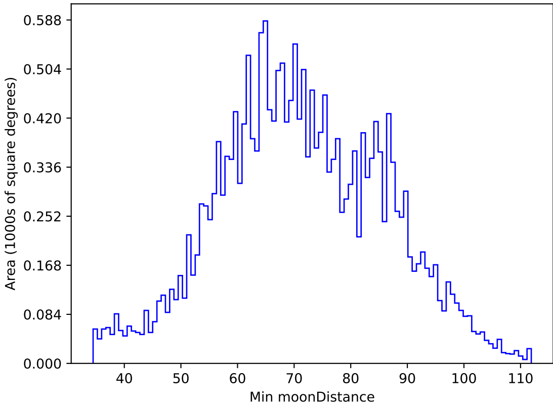
retro_baseline_v2.0_10yrs All sky u band: Min moonDistance
