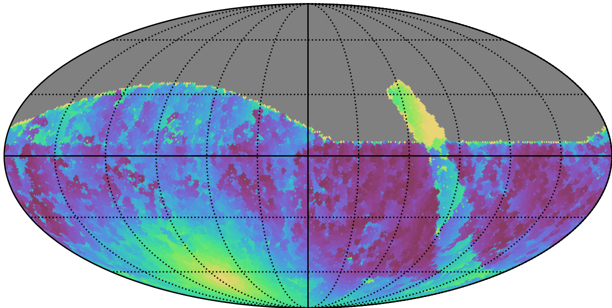
retro_baseline_v2.0_10yrs All sky r band: Min moonDistance
