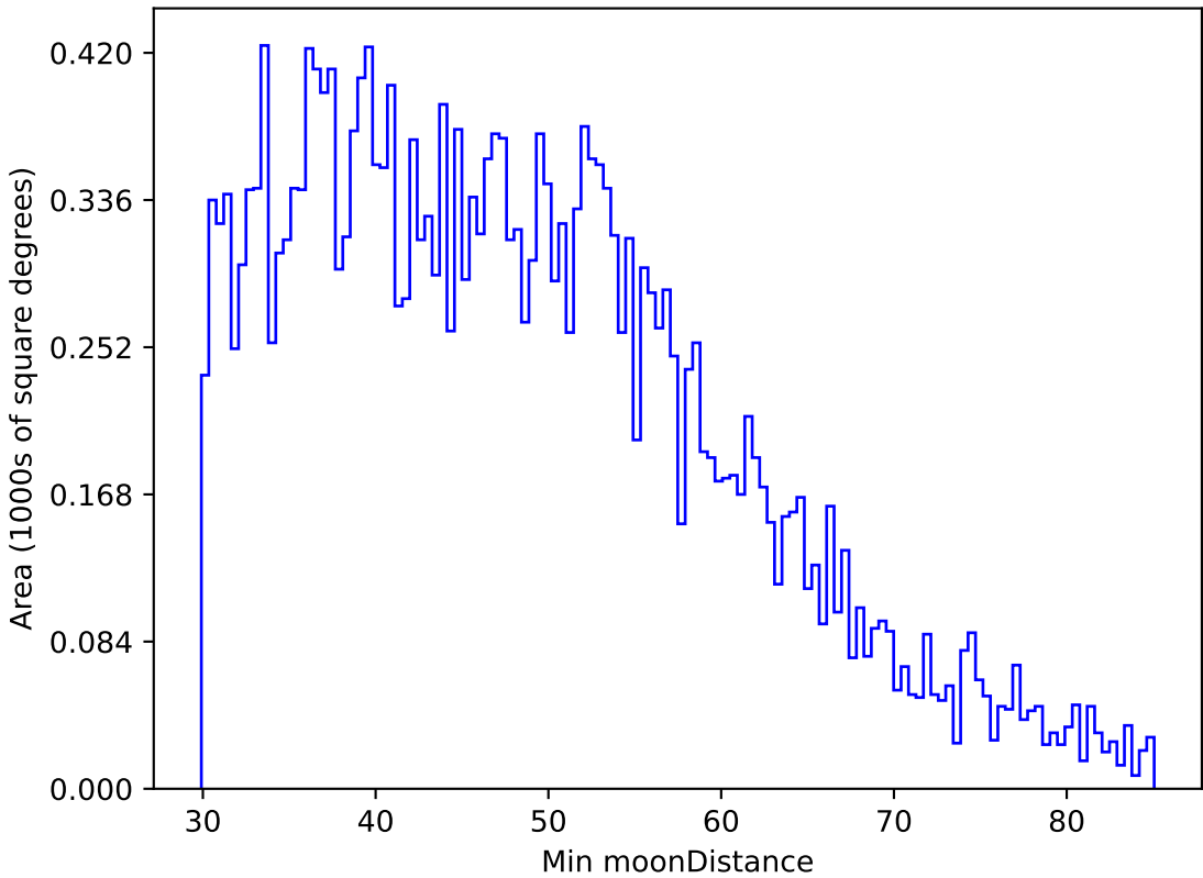
retro_baseline_v2.0_10yrs All sky r band: Min moonDistance
