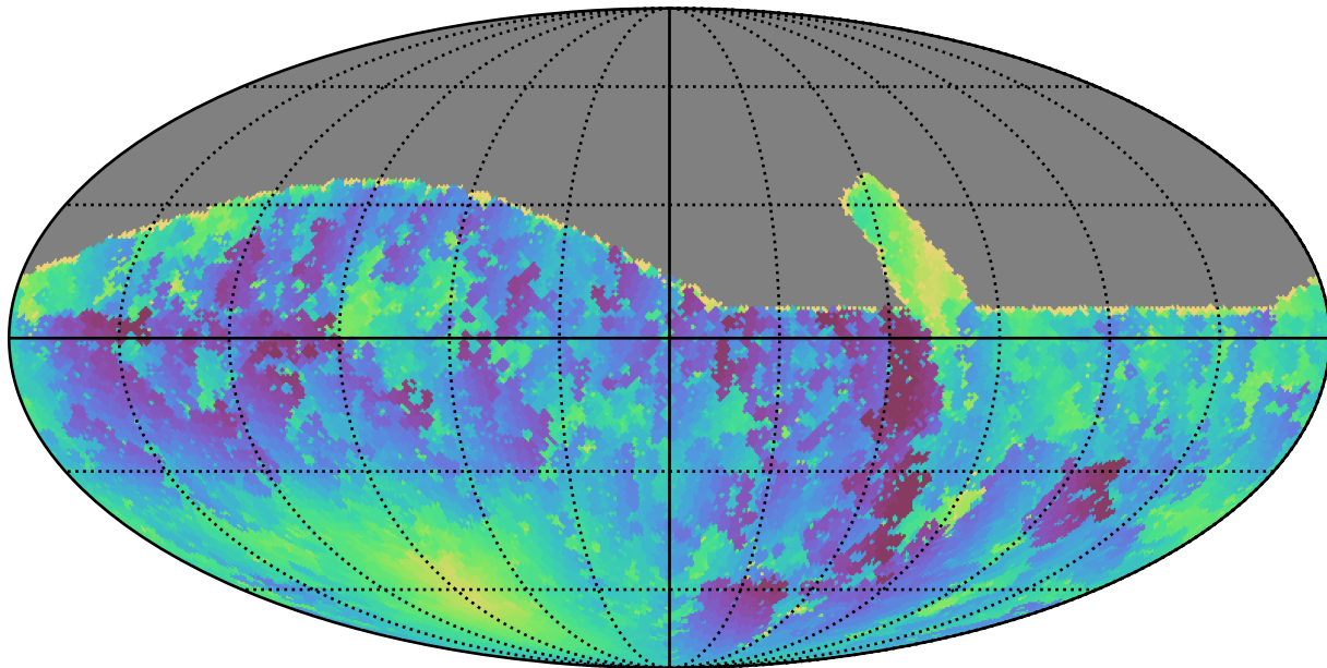
retro_baseline_v2.0_10yrs All sky g band: Min moonDistance
