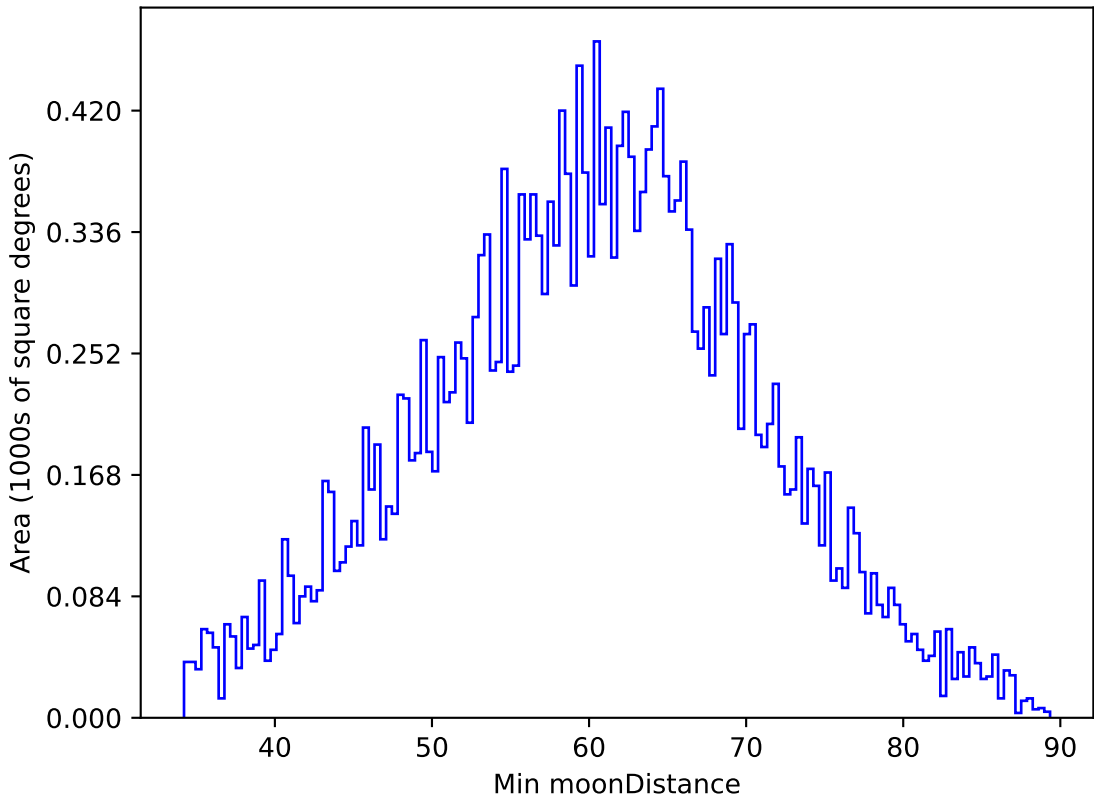
retro_baseline_v2.0_10yrs All sky g band: Min moonDistance
