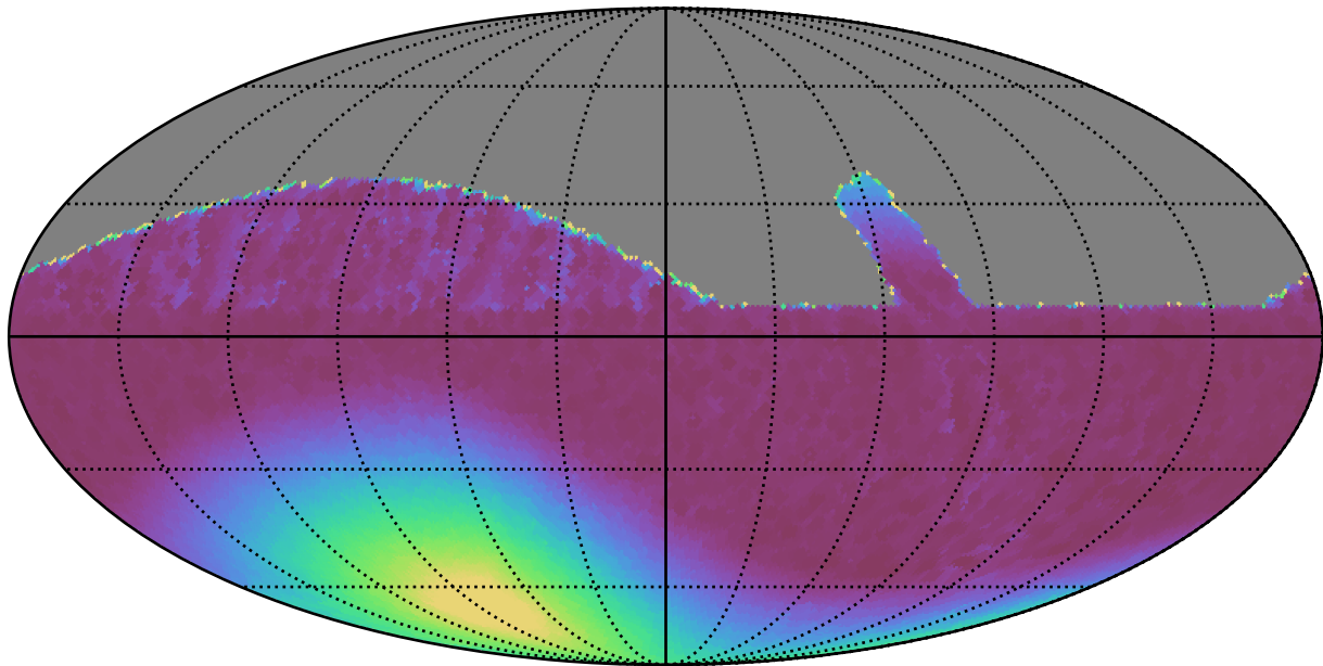
retro_baseline_v2.0_10yrs All sky all bands: Min moonDistance
