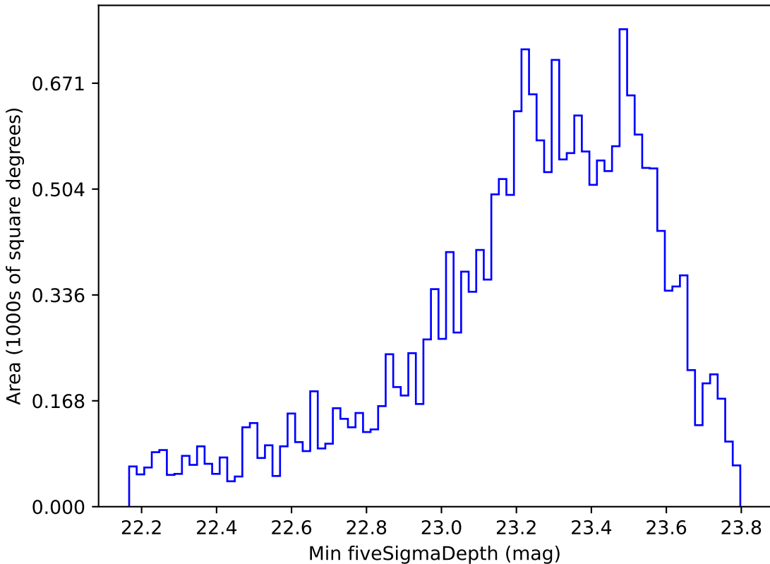
retro_baseline_v2.0_10yrs Yr 1 u band: Min fiveSigmaDepth
