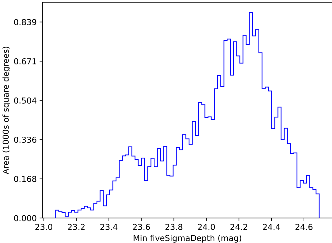
retro_baseline_v2.0_10yrs Yr 1 g band: Min fiveSigmaDepth
