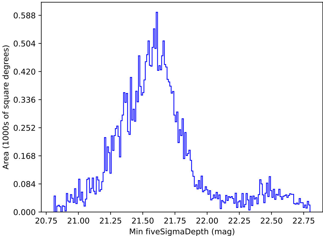
retro_baseline_v2.0_10yrs Yr 1 all bands: Min fiveSigmaDepth
