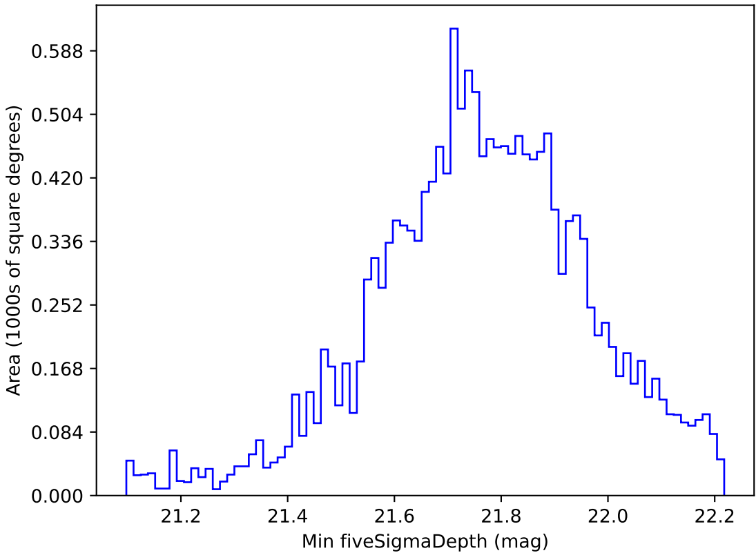
retro_baseline_v2.0_10yrs WFD z band: Min fiveSigmaDepth
