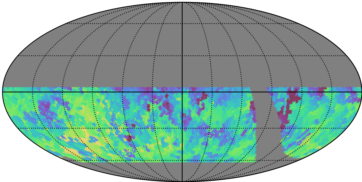
retro_baseline_v2.0_10yrs WFD y band: Min fiveSigmaDepth
