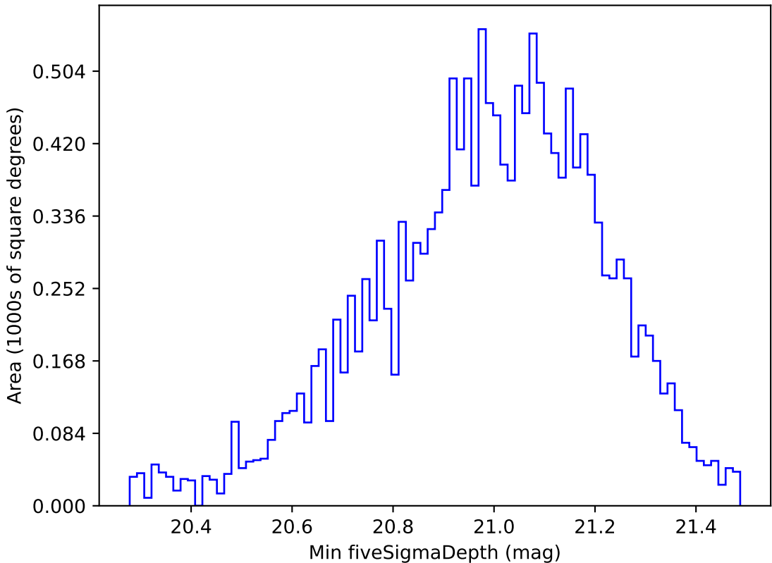
retro_baseline_v2.0_10yrs WFD y band: Min fiveSigmaDepth
