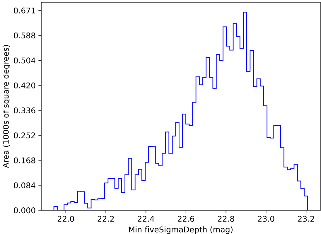
retro_baseline_v2.0_10yrs WFD u band: Min fiveSigmaDepth
