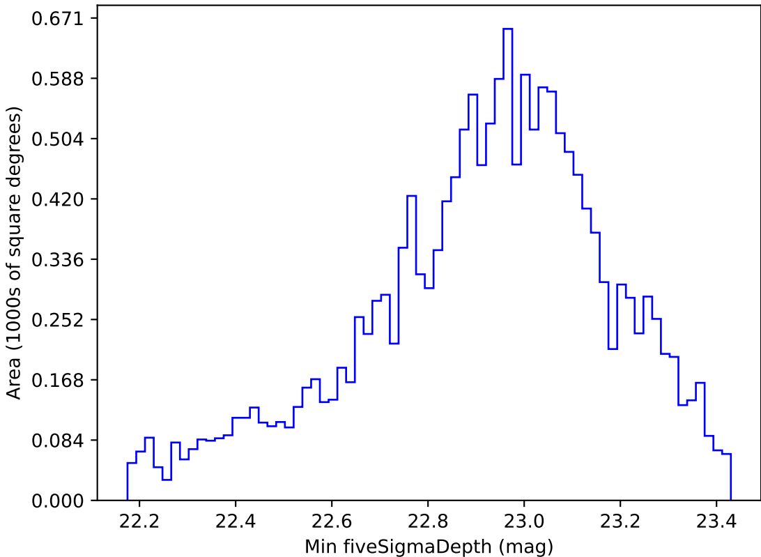
retro_baseline_v2.0_10yrs WFD r band: Min fiveSigmaDepth
