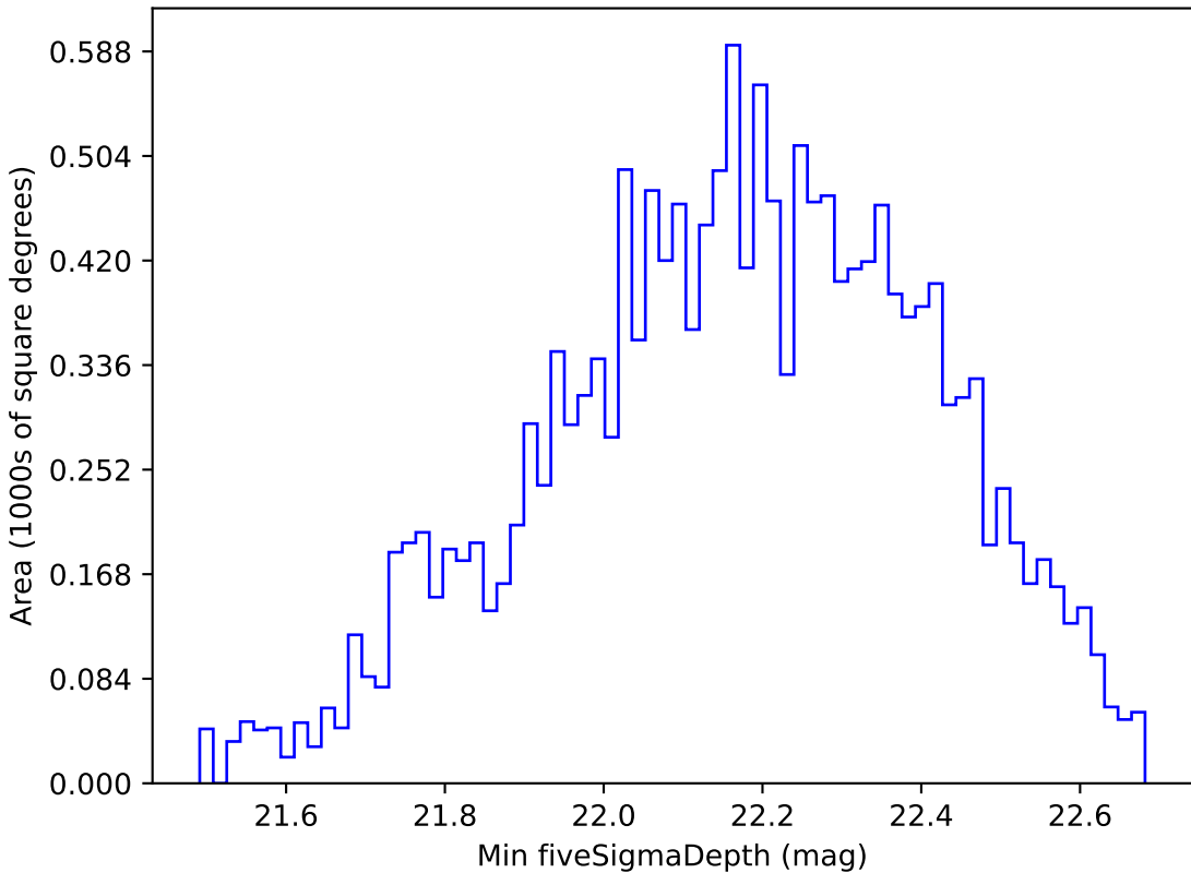
retro_baseline_v2.0_10yrs WFD i band: Min fiveSigmaDepth
