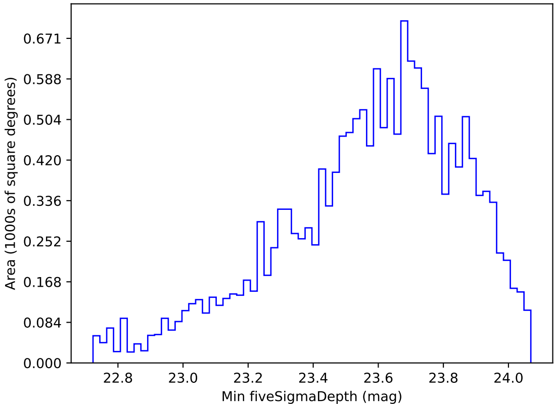
retro_baseline_v2.0_10yrs WFD g band: Min fiveSigmaDepth
