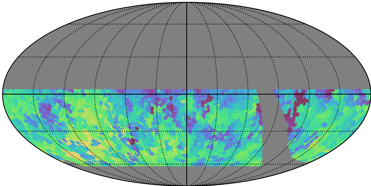
retro_baseline_v2.0_10yrs WFD all bands: Min fiveSigmaDepth
