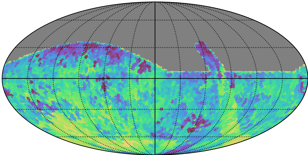
retro_baseline_v2.0_10yrs All sky z band: Min fiveSigmaDepth
