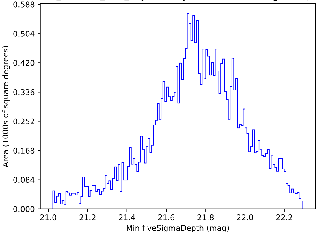
retro_baseline_v2.0_10yrs All sky z band: Min fiveSigmaDepth
