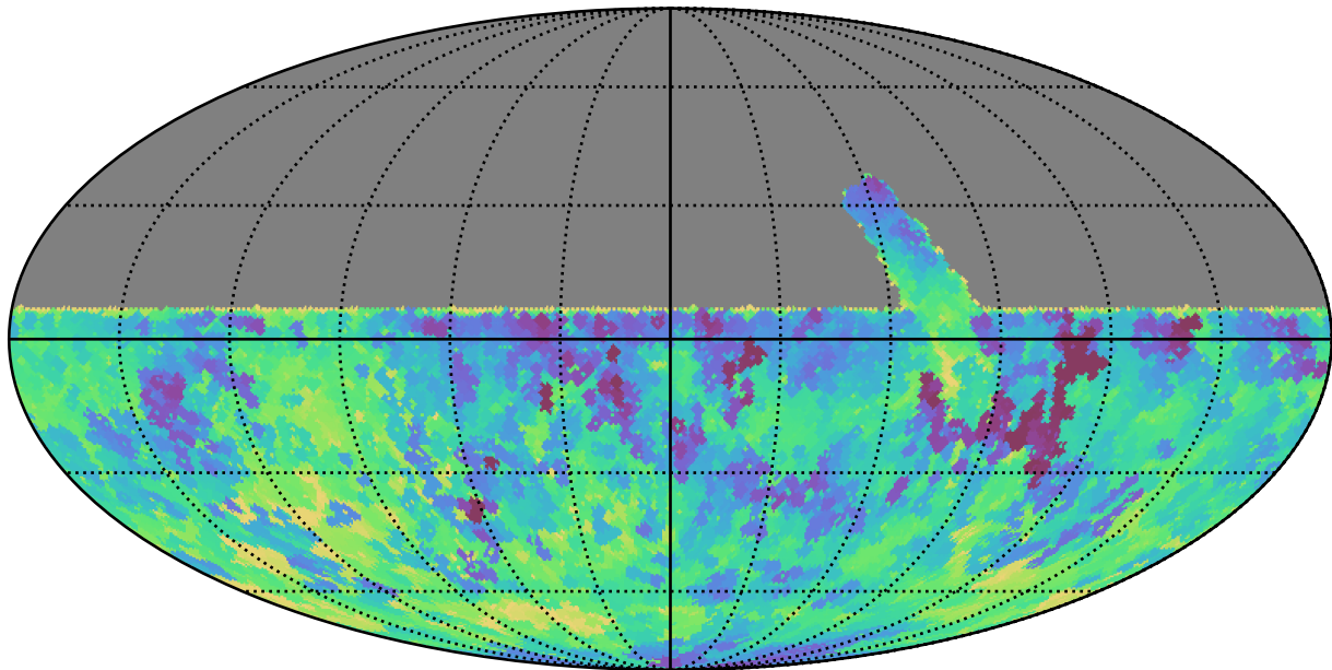
retro_baseline_v2.0_10yrs All sky y band: Min fiveSigmaDepth
