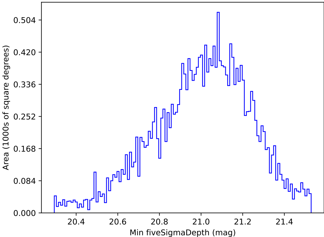
retro_baseline_v2.0_10yrs All sky y band: Min fiveSigmaDepth
