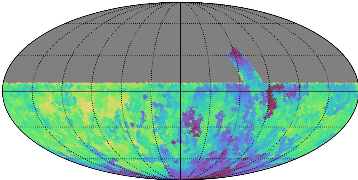
retro_baseline_v2.0_10yrs All sky u band: Min fiveSigmaDepth
