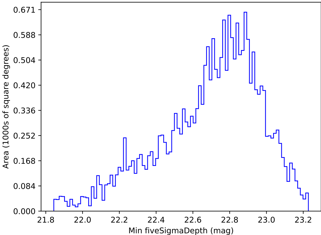
retro_baseline_v2.0_10yrs All sky u band: Min fiveSigmaDepth
