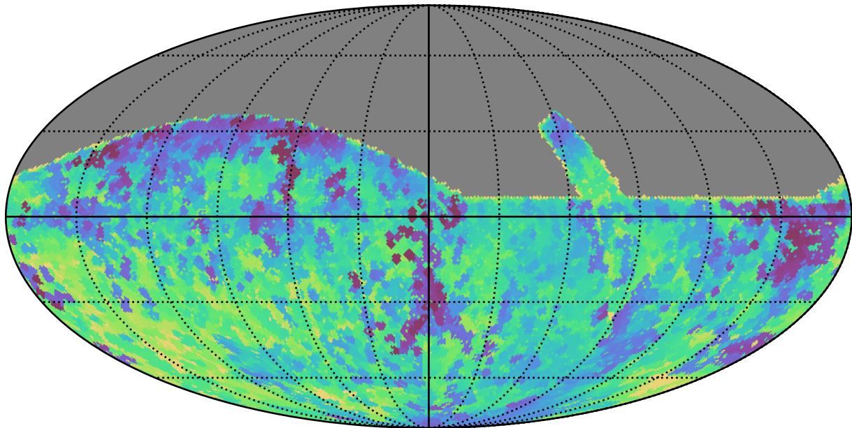
retro_baseline_v2.0_10yrs All sky r band: Min fiveSigmaDepth
