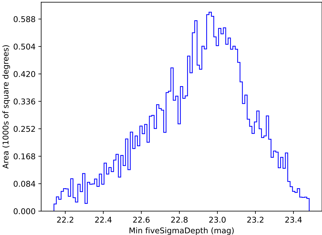
retro_baseline_v2.0_10yrs All sky r band: Min fiveSigmaDepth
