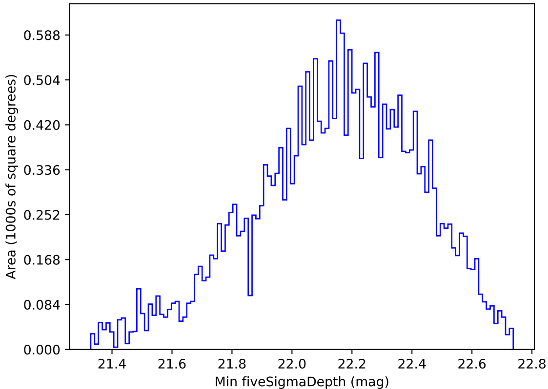
retro_baseline_v2.0_10yrs All sky i band: Min fiveSigmaDepth
