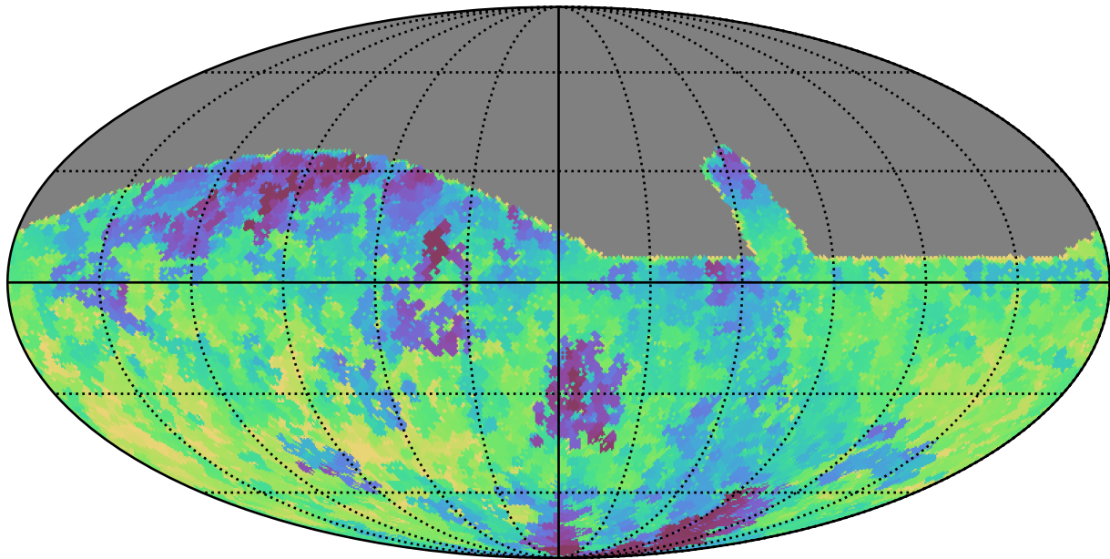
retro_baseline_v2.0_10yrs All sky g band: Min fiveSigmaDepth
