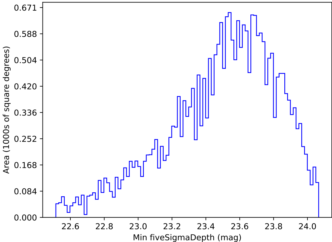
retro_baseline_v2.0_10yrs All sky g band: Min fiveSigmaDepth
