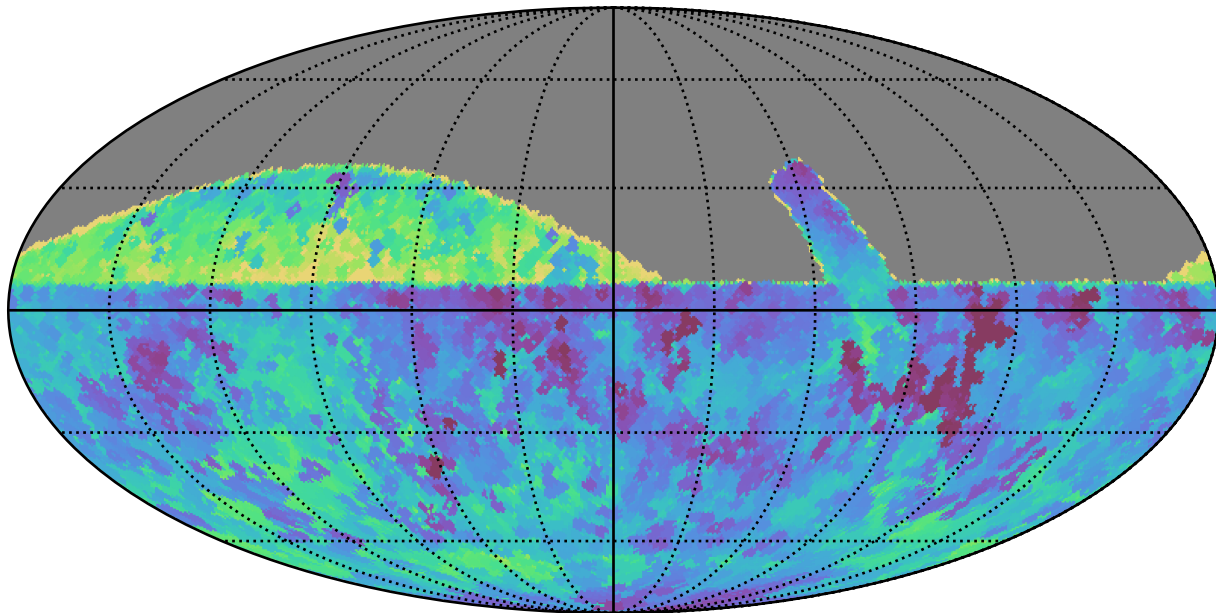
retro_baseline_v2.0_10yrs All sky all bands: Min fiveSigmaDepth
