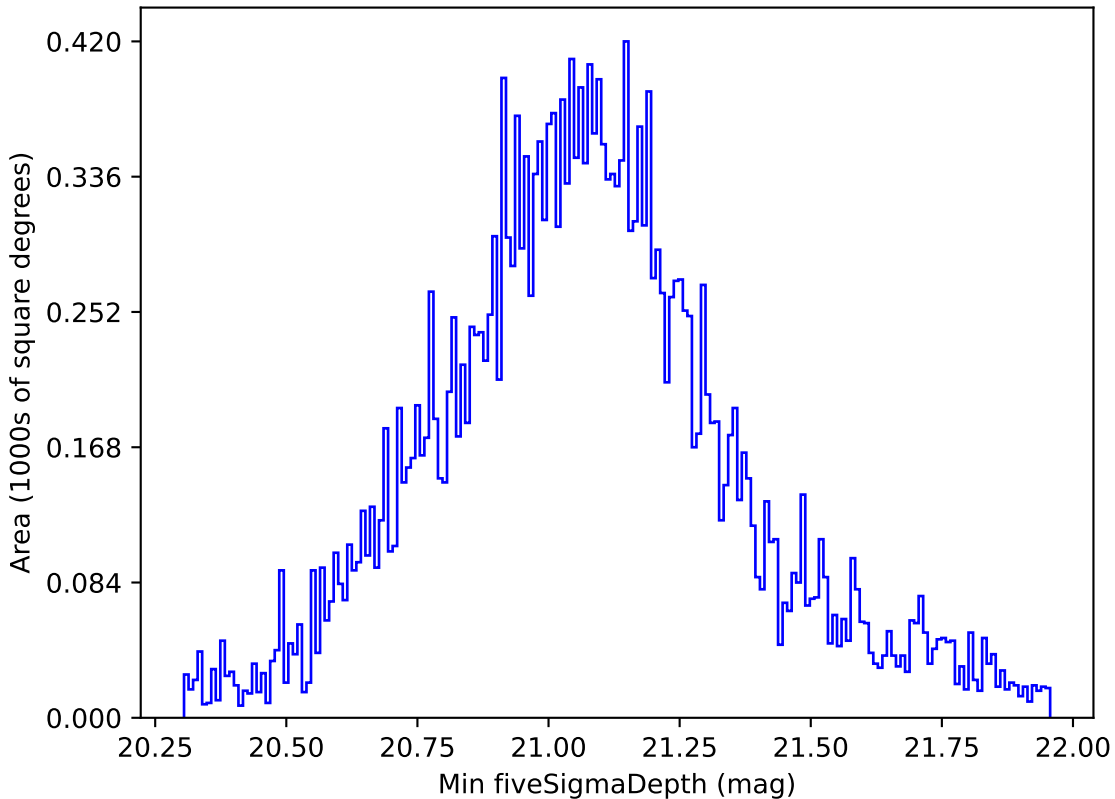
retro_baseline_v2.0_10yrs All sky all bands: Min fiveSigmaDepth
