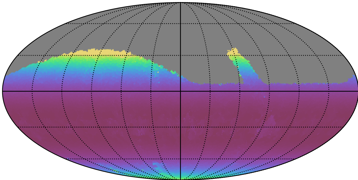
retro_baseline_v2.0_10yrs Yr 1 z band: Min airmass
