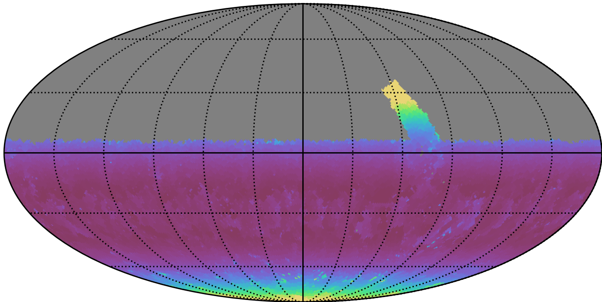
retro_baseline_v2.0_10yrs Yr 1 u band: Min airmass
