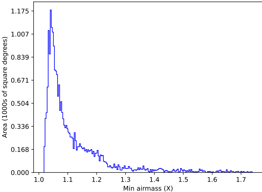
retro_baseline_v2.0_10yrs Yr 1 u band: Min airmass
