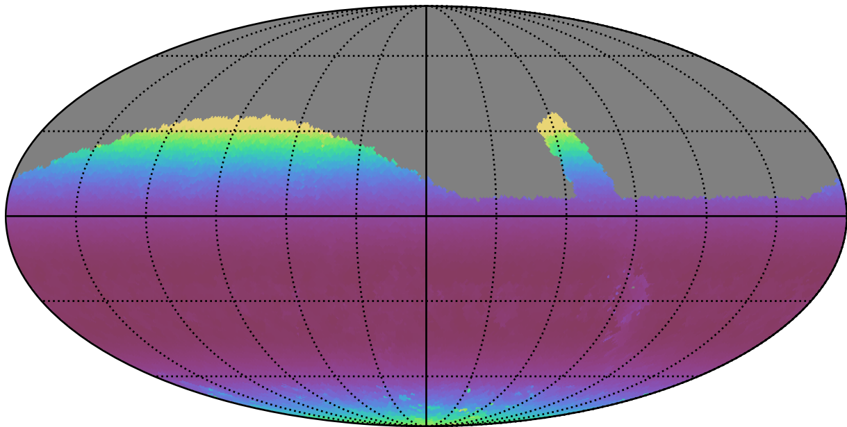
retro_baseline_v2.0_10yrs Yr 1 r band: Min airmass
