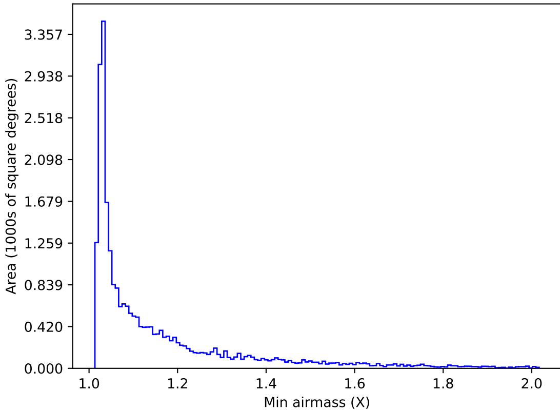
retro_baseline_v2.0_10yrs Yr 1 r band: Min airmass
