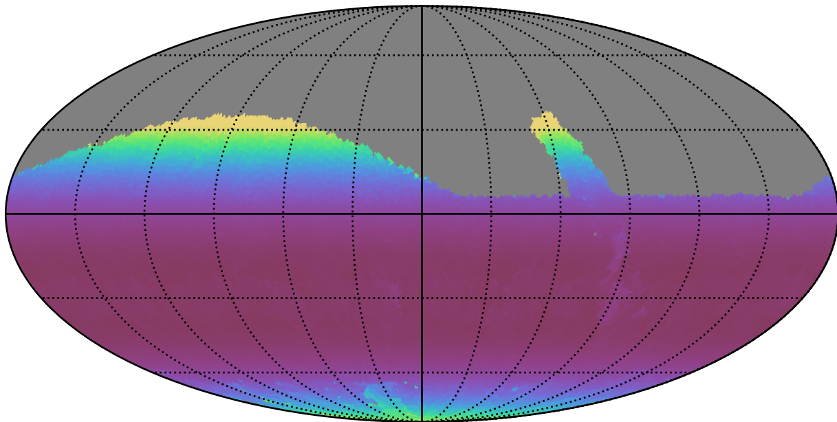
retro_baseline_v2.0_10yrs Yr 1 i band: Min airmass
