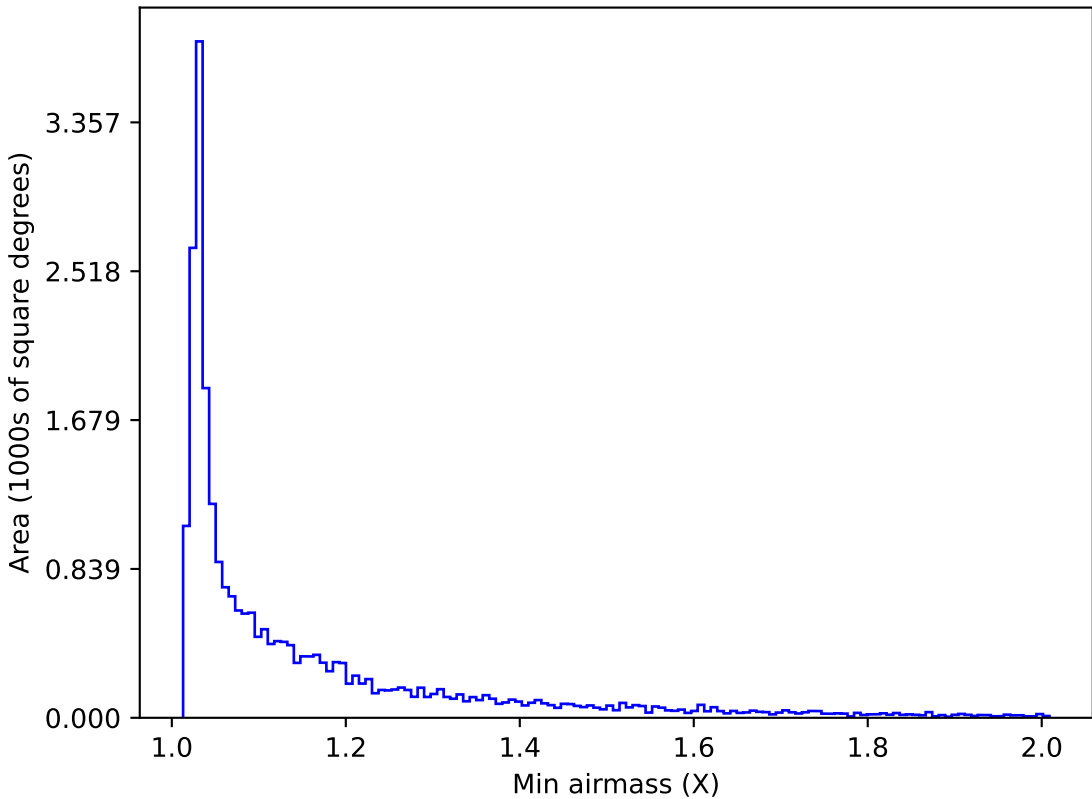
retro_baseline_v2.0_10yrs Yr 1 i band: Min airmass
