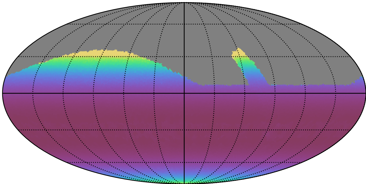
retro_baseline_v2.0_10yrs Yr 1 all bands: Min airmass
