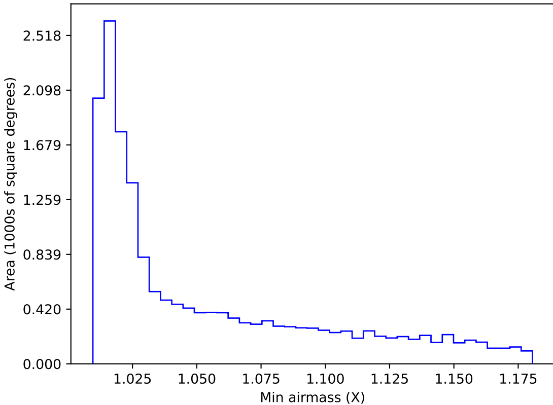
retro_baseline_v2.0_10yrs WFD z band: Min airmass
