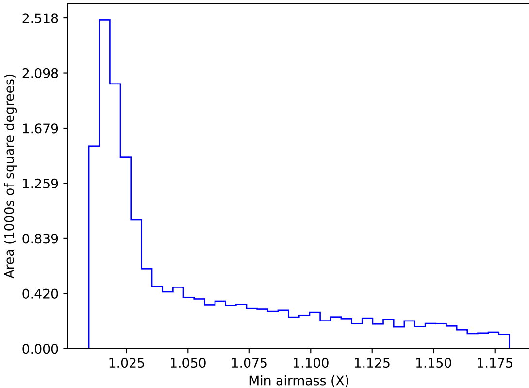
retro_baseline_v2.0_10yrs WFD y band: Min airmass
