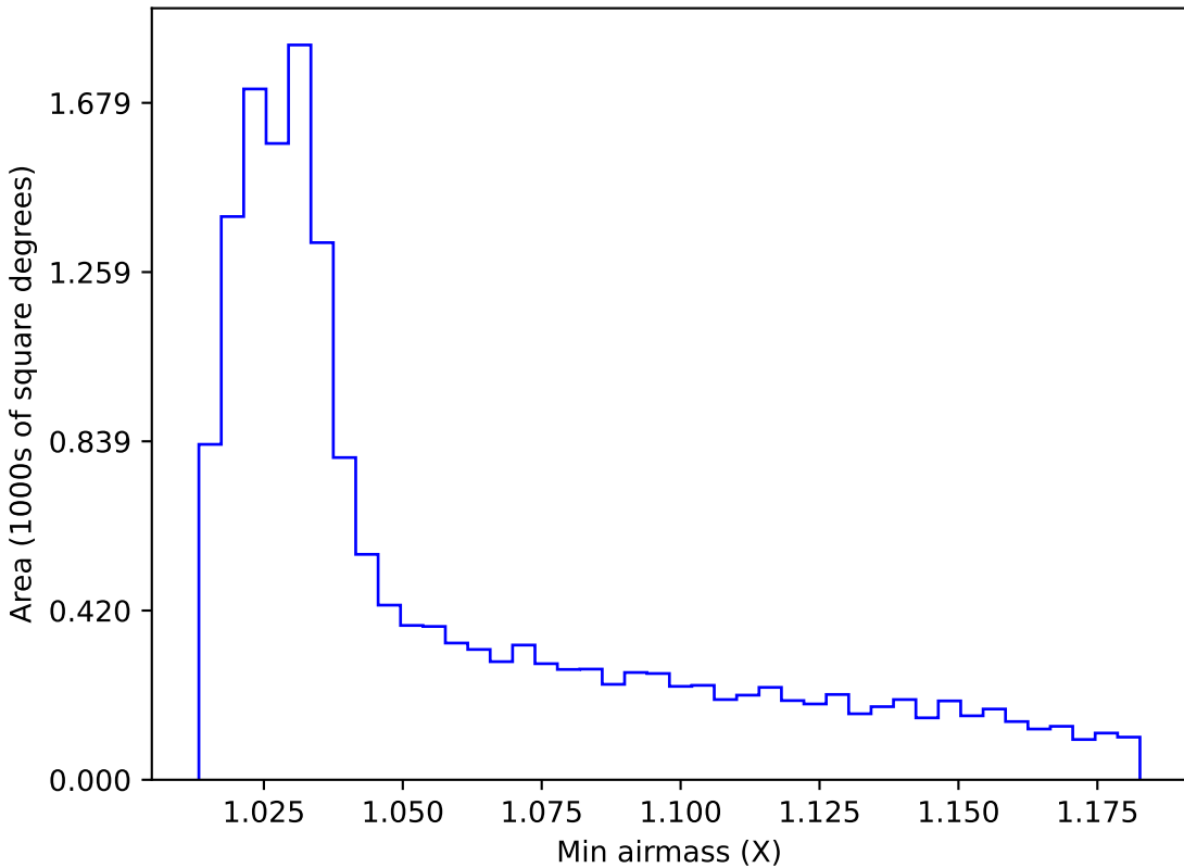
retro_baseline_v2.0_10yrs WFD u band: Min airmass
